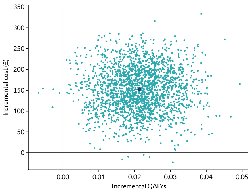
FIGURE 18 The PSA results on a cost-effectiveness plane.
