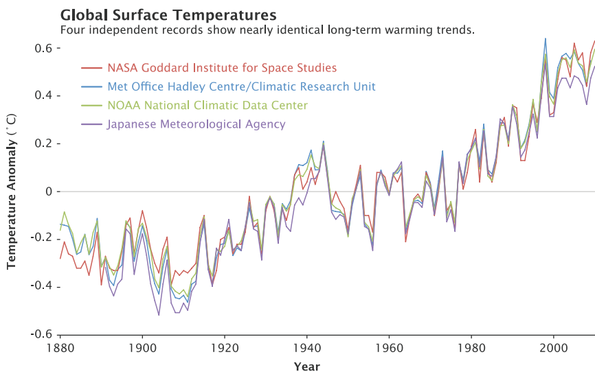
FIGURE A17-2 A comparison of the existing four global surface temperature datasets that are used in climate analyses. These datasets are based on the same input data and differ by interpolation among stations, treatment of missing data, and the length of the record. The data in this figure have been adjusted to a common baseline period.
