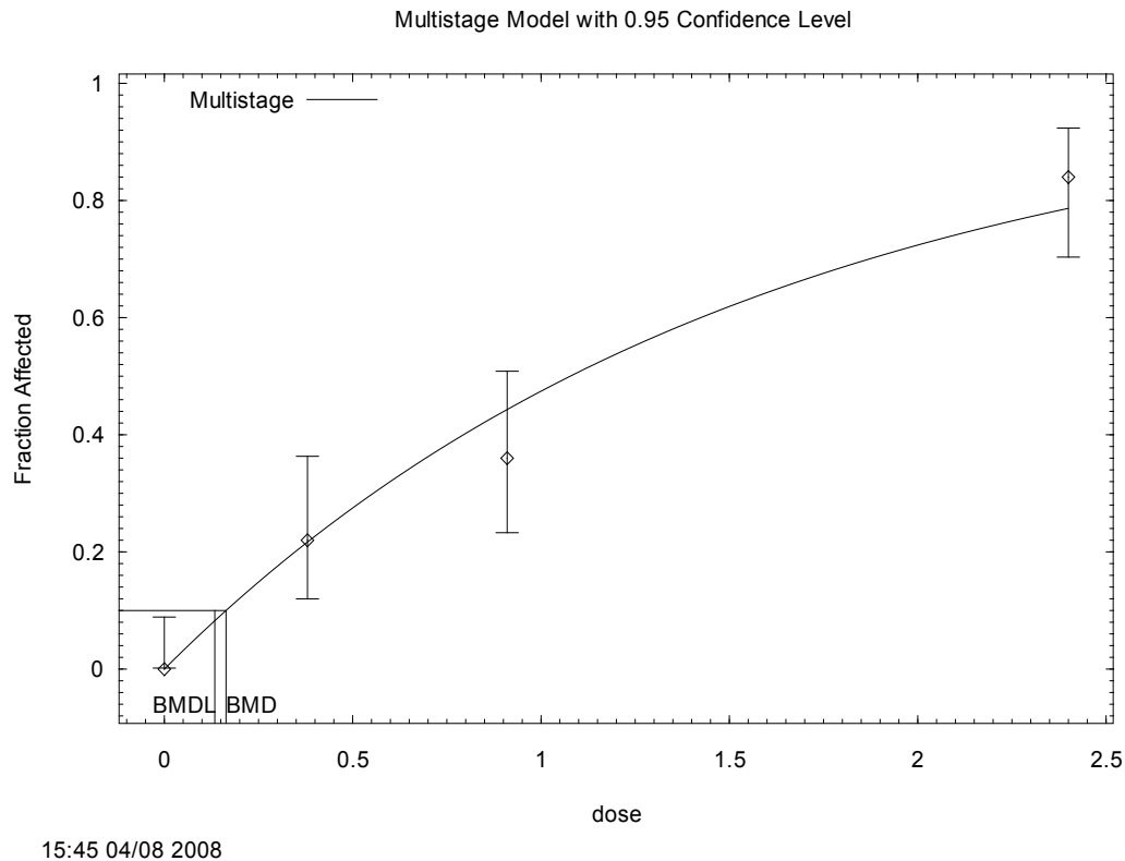
Figure A-5. Predicted and Observed Incidence of Diffuse Epithelial Hyperplasia in the Duodenum of Male Mice Exposed to Sodium Dichromium Dihydrate in Drinking Water for 2 Years*
