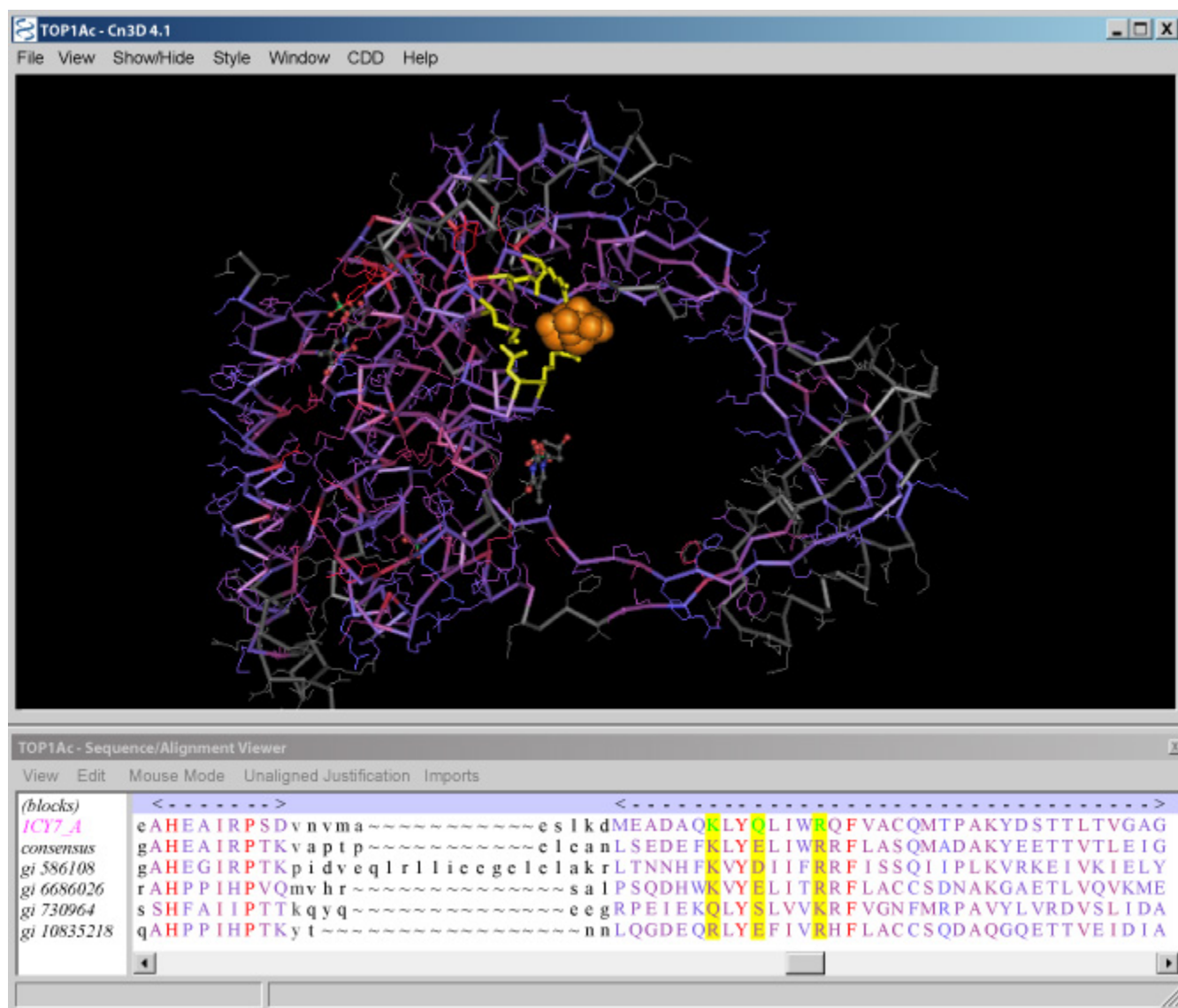
Figure 7. Sequence and structure views of the TOPIAc conserved domain common to type III bacterial and eukaryotic DNA topoisomerases. The upper window displays the structure of the domain with the residues colored according to their sequence conservation, with red indicating high conservation and blue indicating low conservation. The nucleotide bound at site II is shown as an orange space-filling model, and the residues involved in this binding site are yellow . The lower window displays the sequence alignment for the domain with aligned residues shown as colored capital letters . Residues aligned to three of the binding site residues are highlighted in yellow . The sequence for NP_004609 (gi 10835218) occupies the bottom row .
